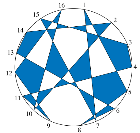
The (17, 7) residue design
