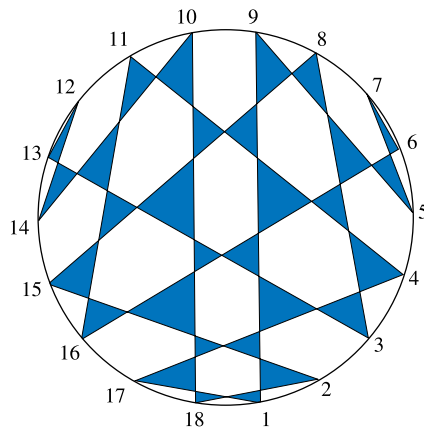
The (19, 9) residue design
