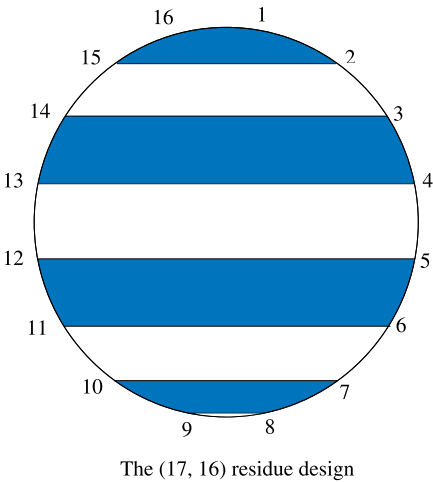
The (17, 16) residue design
