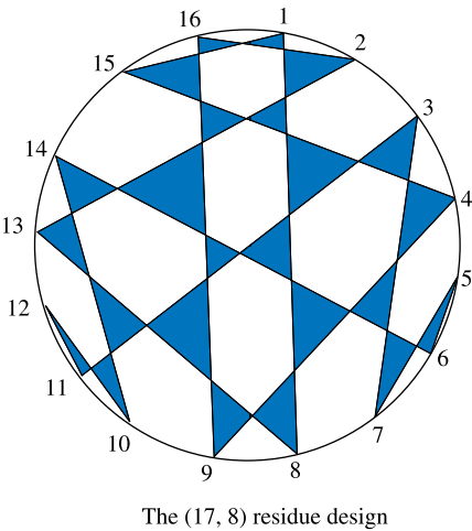
The (17, 8) residue design
